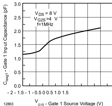
Figure 5. Gate 1 Input Capacitance vs. Gate 1 Source Voltage
