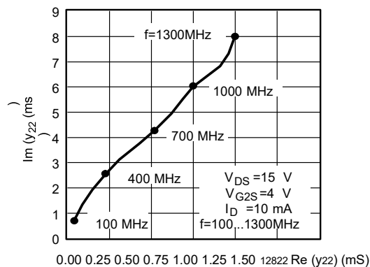
Figure 11. Short Circuit Output Admittance
