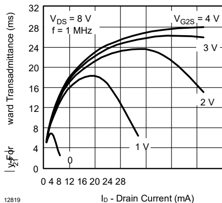
Figure 8. Forward Transadmittance vs. Drain Current
