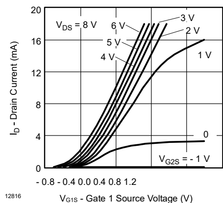
Figure 3. Drain Current vs. Gate 1 Source Voltage
