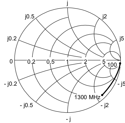
Figure 15. Output Reflection Coefficient
